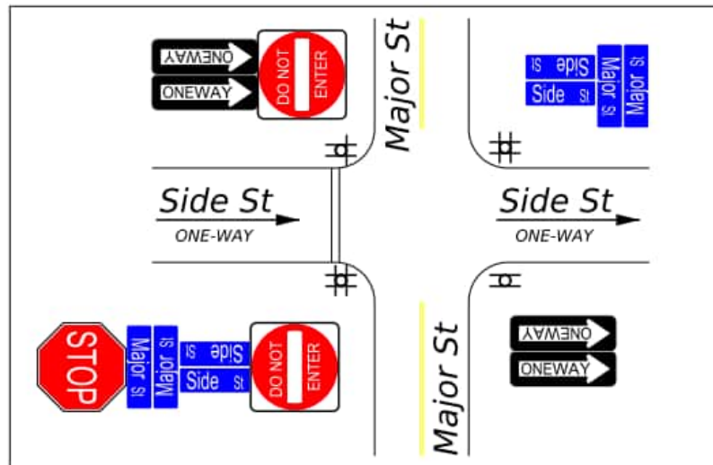
Figure 6.1: Sign Layout for Stopped Controlled Intersection Example #1
